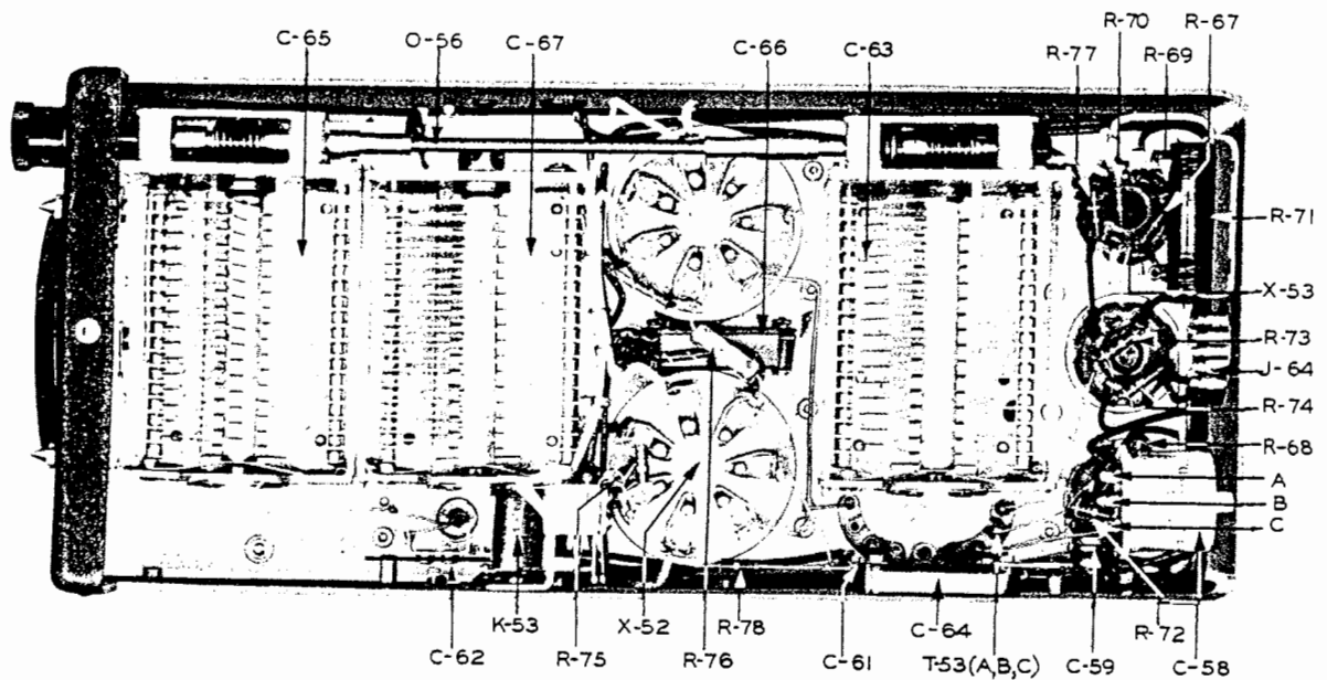
FIGURE 14—TYPICAL RADIO TRANSMITTER, BOTTOM VIEW WITH COVER REMOVED
