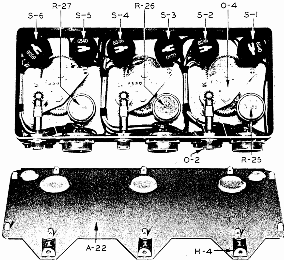
FIGURE 9B—RADIO CONTROL BOX BC-450-A, REAR VIEW WITH COVER REMOVED
