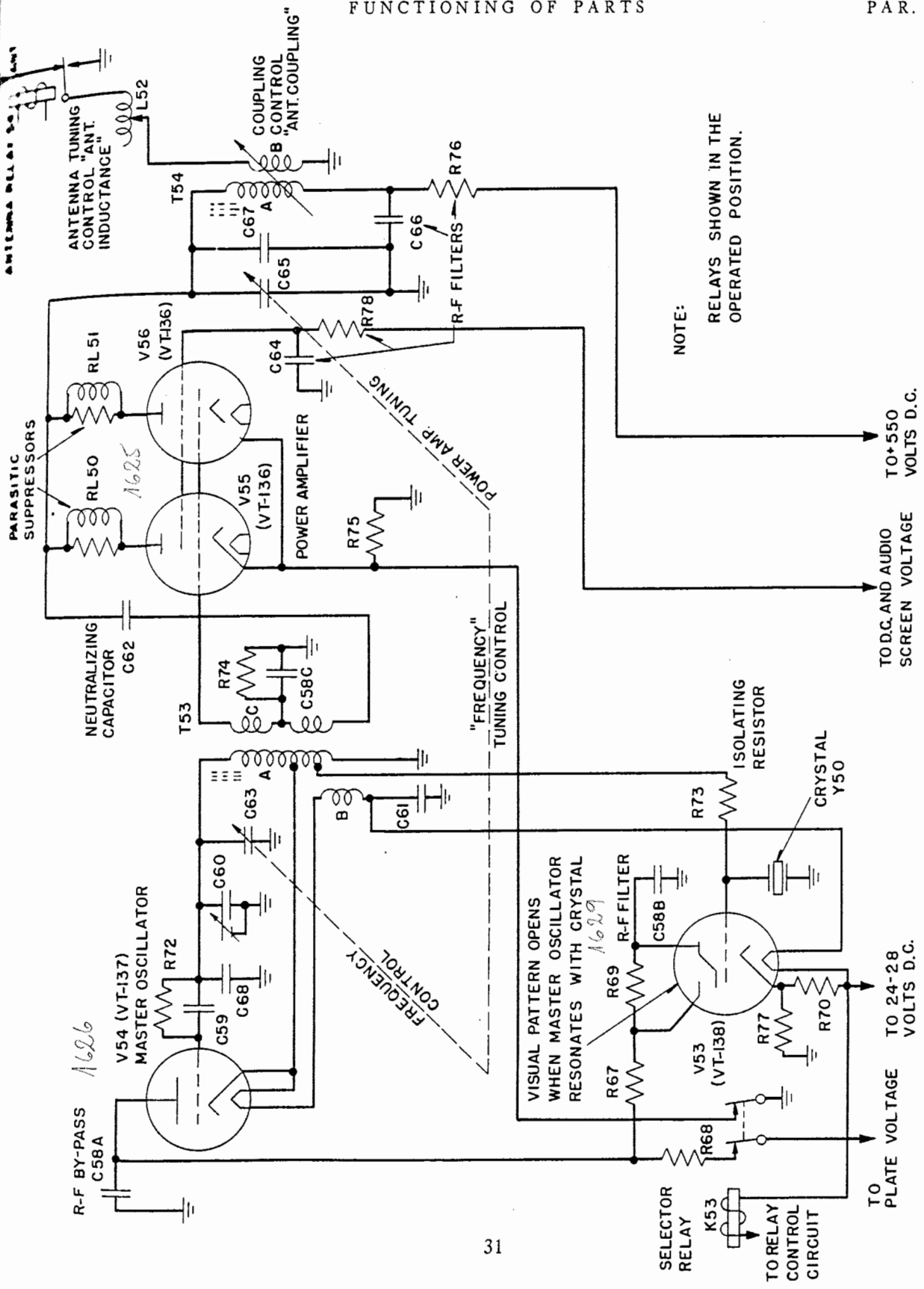
FIGURE 12.—FUNCTIONAL DIAGRAM OF THE R-F CIRCUITS OF A TYPICAL RADIO TRANSMITTER
