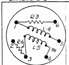
RF COIL SET SYMBOL Z-5
