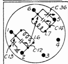
IF COUPLING UNITS
