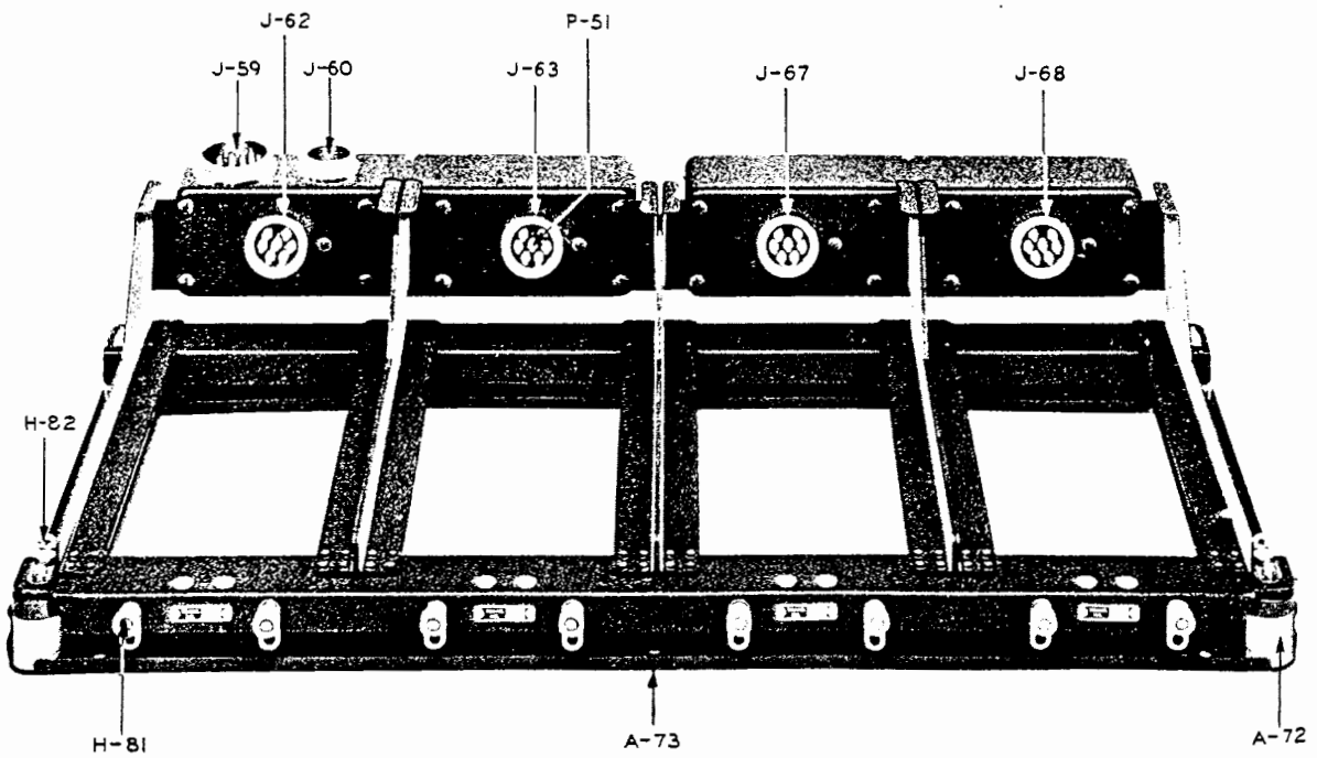
FIGURE 17B—RACK FT-331-A AND MOUNTING FT-332-A, FRONT VIEW
