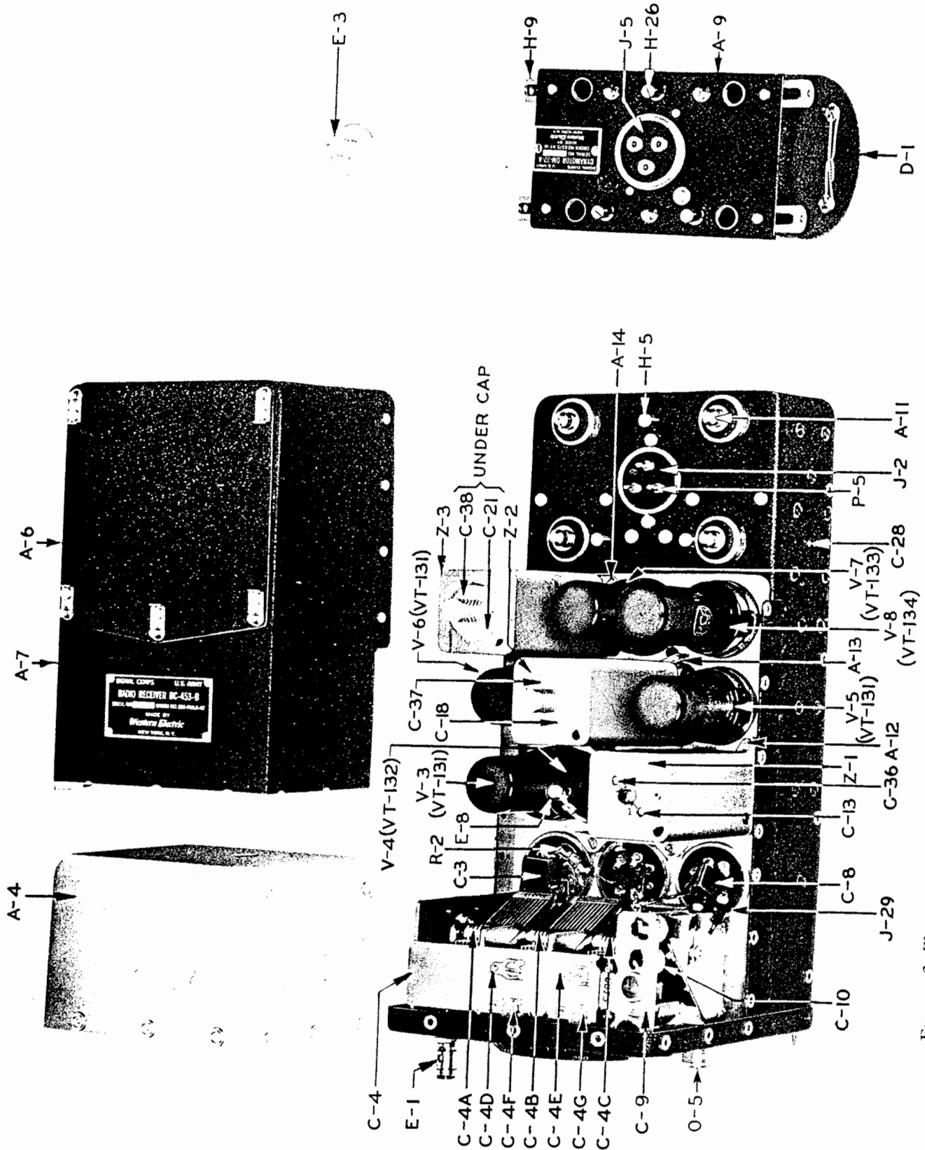
FIGURE 3—TYPICAL RADIO RECEIVER, TOP INSIDE VIEW, AND BOTTOM VIEW OF DYNAMOTOR DM-32-A
