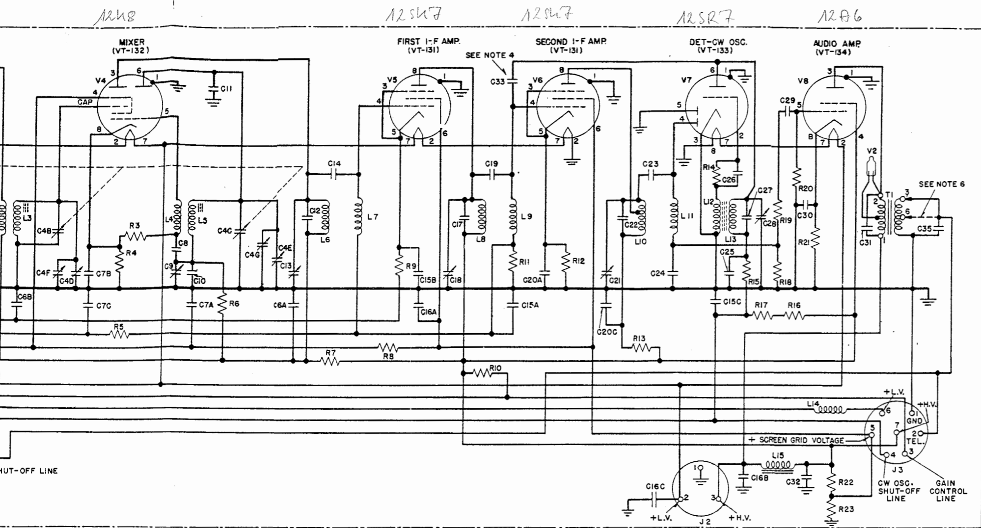
TYPICAL RADIO RECEIVER BC-455-B (6-9.1 MC). I-F = 2830 KC
