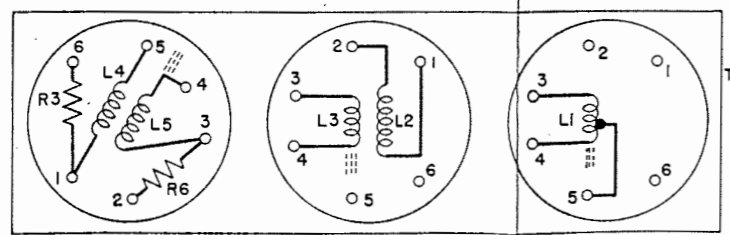
DETAIL SCHEMATIC DIAGRAMS COIL ASSEMBLIES AND TRANSFORMERS
