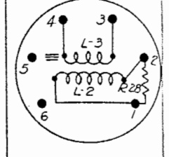
SYMBOL Z-5B RF AMPLIFIER
