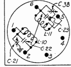
SYMBOL Z-3 3RD I.F. (239 KC)
