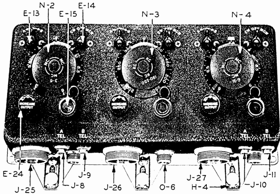
FIGURE 9A—RADIO CONTROL BOX BC-450-A, FRONT VIEW
