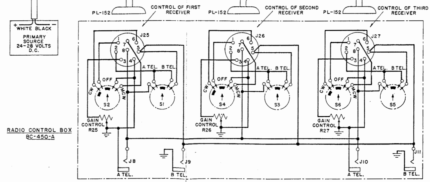
FIGURE 26-RADIO SET SCR-274-N RECEIVING EQUIPMENT, SCHEMATIC CIRCUIT DIAGRAM
