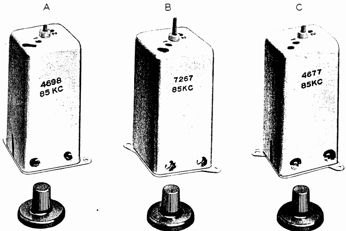
FIGURE 25—TYPICAL I-F COUPLING UNIT ASSEMBLIES
