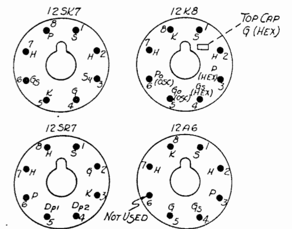
TUBE TERMINAL CODE
