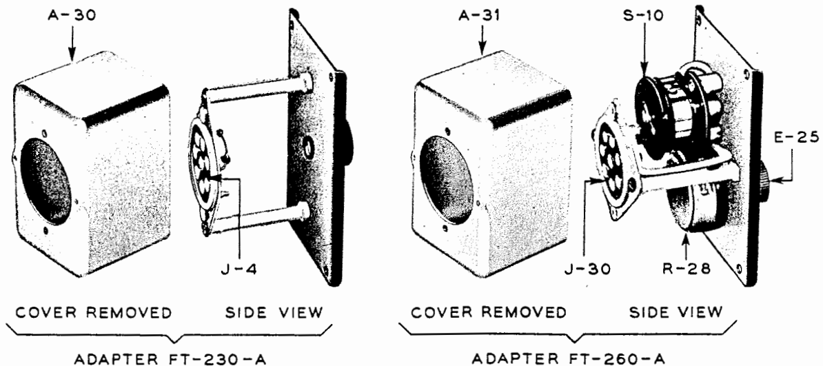
FIGURE 6—ADAPTERS FT-230-A AND FT-260-A
