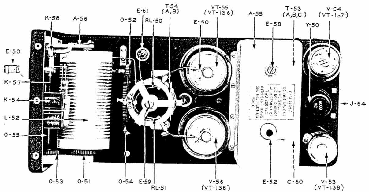
FIGURE 13—TYPICAL RADIO TRANSMITTER, TOP VIEW WITH SHIELD REMOVED
