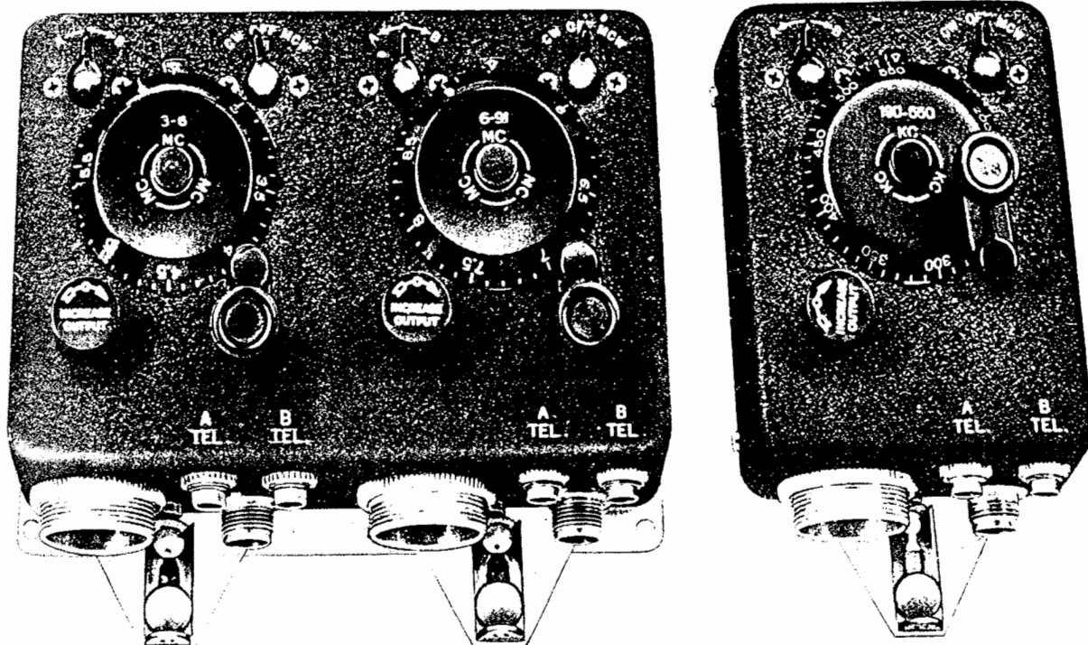
FIGURE 10—LEFT, RADIO CONTROL BOX BC-496-A (FOR TWO RECEIVERS); RIGHT, RADIO CONTROL BOX BC-473-A (OR -B) (FOR ONE RECEIVER)
