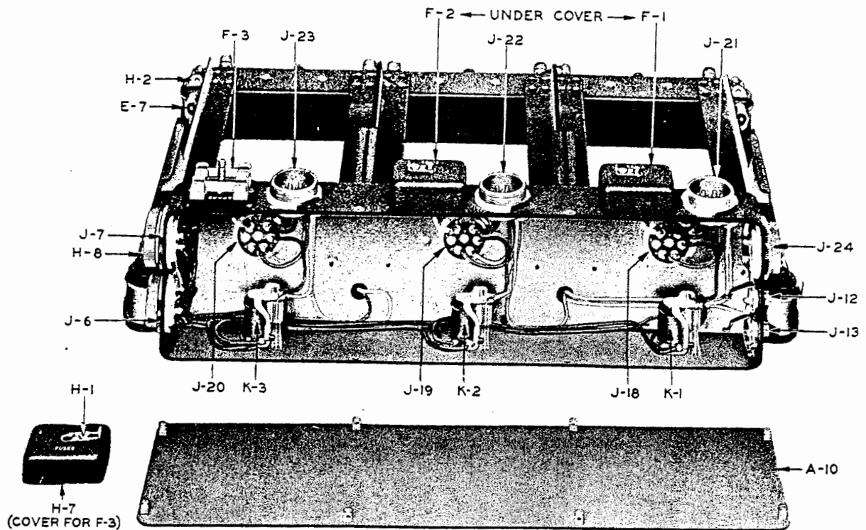
FIGURE 7B—RACK FT-220-A AND MOUNTING FT-221-A, REAR VIEW WITH COVER OF RACK REMOVED
