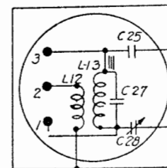
SYMBOL Z-4 CW OSCILLATOR (239 KC)
