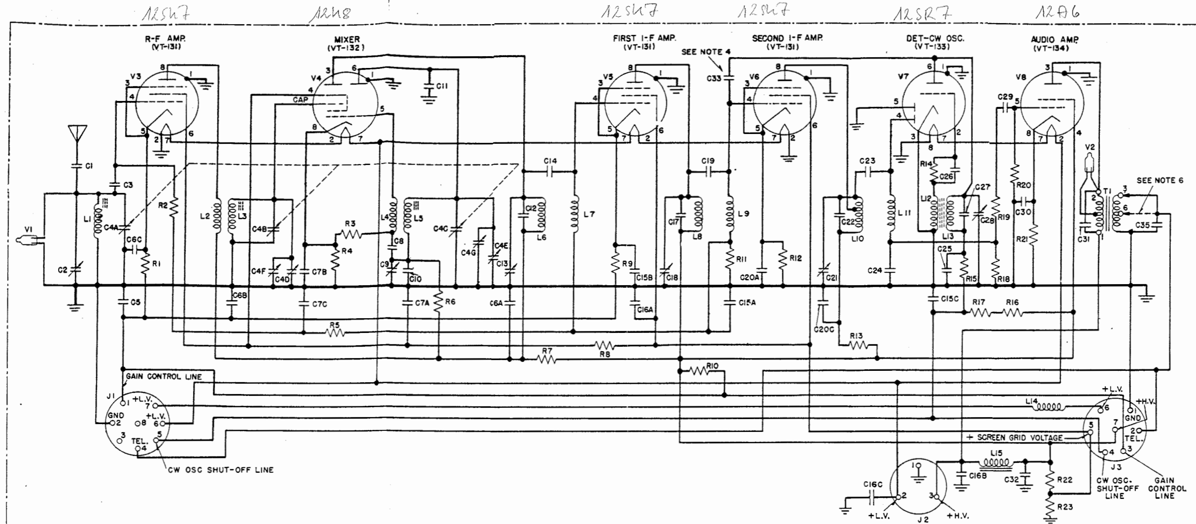
TYPICAL RADIO RECEIVER BC-455-B (6-9.1 MC). I-F = 2830 KC
