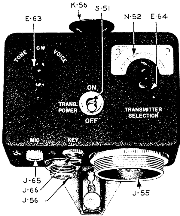
FIGURE 19A—RADIO CONTROL BOX BC-451-A, FRONT VIEW
