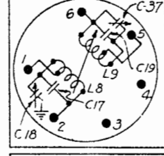
SYMBOL Z-2 2ND I.F. (239 KC)
